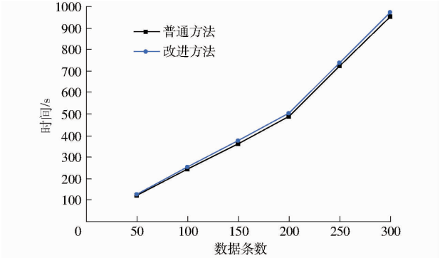
图 4 普通方法和改进方法在不同数据条数下保存数据时间对比 Fig. 4 Comparison of data saving time of common method and improved method under different data pieces
