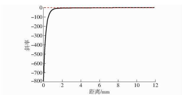
图 10 缺口应力场拟合曲线斜率 Fig.10 Slope of notch stress field distribution fitting curve
