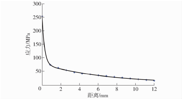
图 9 缺口应力场分布拟合曲线 Fig.9 Fitting curve of notch stress field distribution
