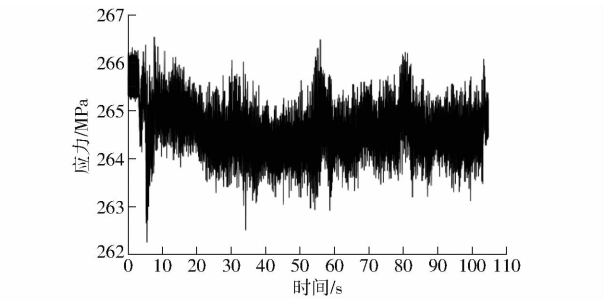
图 8 测点 4 实测载荷-时间历程曲线 Fig.8 Measured load-time curve at measuring point 4
