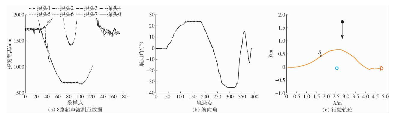
图 20 AGV 绕行 1 个静态障碍物并躲避 1 个动态障碍物的避障试验数据 Fig. 20 Obstacle avoidance test data when AGV detoured a small static obstacle and avoided a dynamic obstacle
