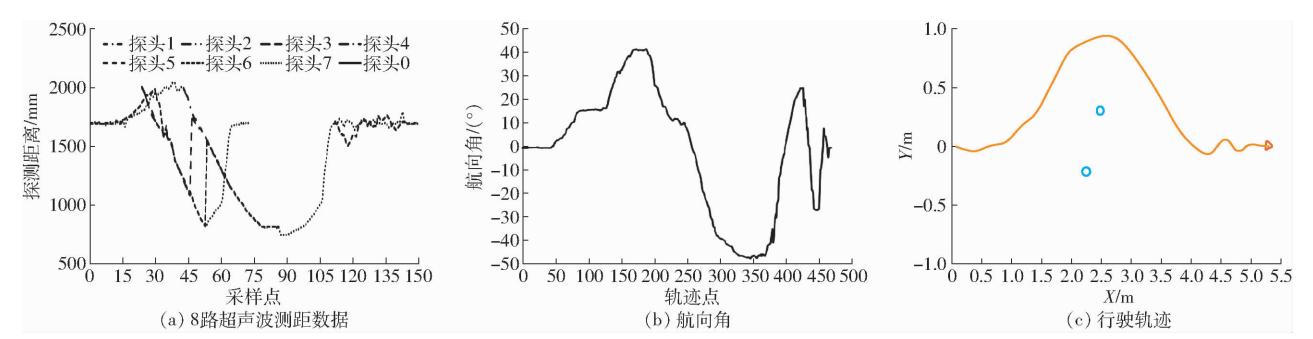
图 19 AGV 连续绕行 2 个小间距静态障碍物的避障数据 Fig. 19 Obstacle avoidance data when AGV detoured continuously two small space static obstacles
