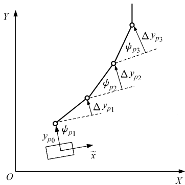
图3 分段计算横向位置差值 Fig.3 Small sections method for lateral position difference calculation
